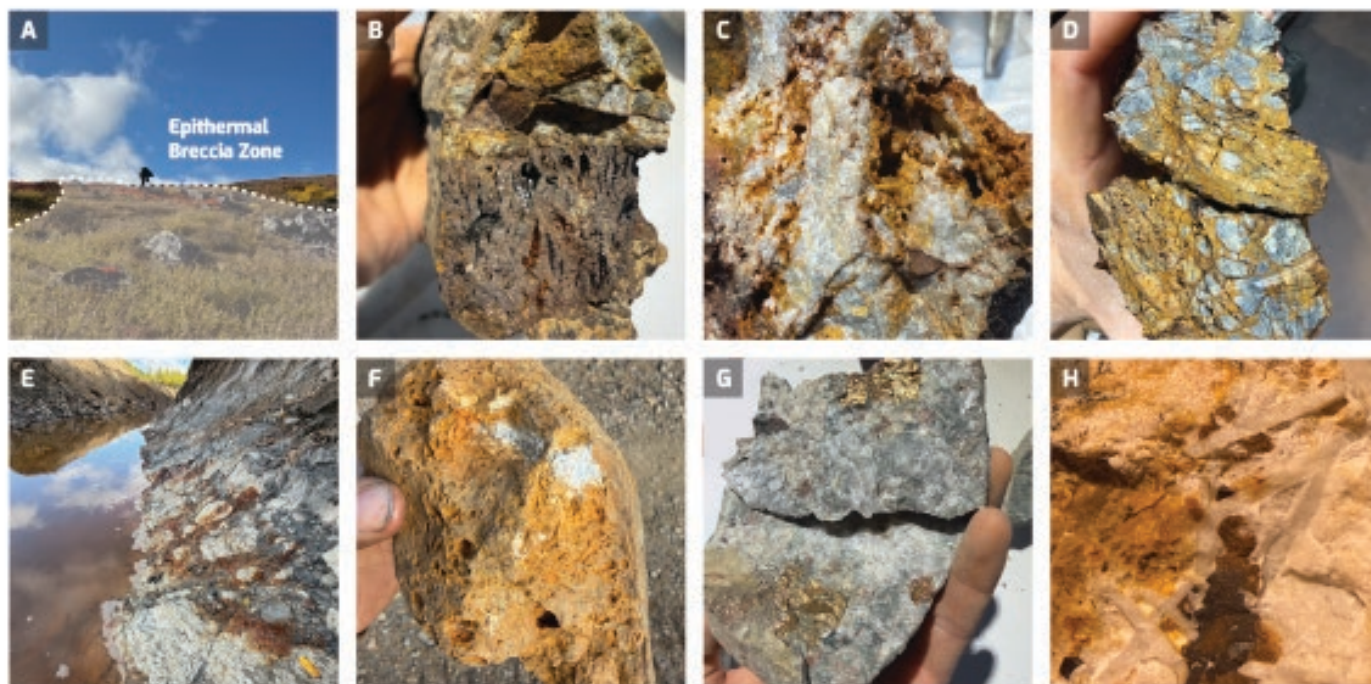
Figure 1. Selected field observations from the 2026 exploration program. A) Newly identified brecciated quartz- vein corridor from Drake claims; B) bladed, drusy quartz pseudomorphs within a gossanous vein hosted in silicified, sericite altered schist on the Drake claims; C) drusy-lined vugs in a recrystallized chalcedonic quartz vein showing intense limonite weathering; D) sample of brecciated, silicified schist from one of the newly identified distal low-sulphidation epithermal corridors at Drake; E) newly exposed clay-altered lithocap at the mouth of Miller Creek, with preserved narrow, feldspar-porphyritic volcanic stockwork-style dykes; F) newly identified sulphide-bearing textures interpreted to be associated with high-sulphidation epithermal alteration at the confluence of Miller Creek and the Sixtymile River; G) potassium feldspar-bearing quartz vein containing large chalcopyrite crystals, discovered in a region of intense D4 deformation; H) close up of low-sulphidation bladed quartz laths identified in clay-filled oxidized veins from the newly staked Sixty claims. High-Resolution Image .
